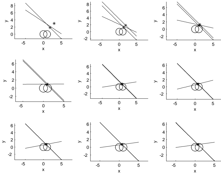
Geometric illustration of Algorithm 3.1 in each iterative step, i.e., the discs and the three half-spaces C_1^n , C_2^n and W^n , with the starting point x^1 = (3, 3)
